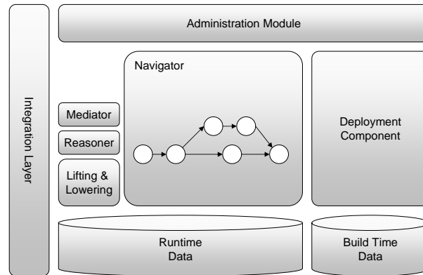
Figure 5. Architecture of a BPEL4SWS Engine.
