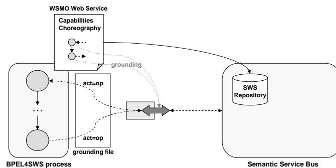
Figure 1. Semantic Synchronous Invocation of a BPEL4SWS process.
