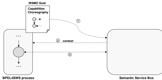
Figure 3. Synchronous Invocation of a WSMO Web Service.
