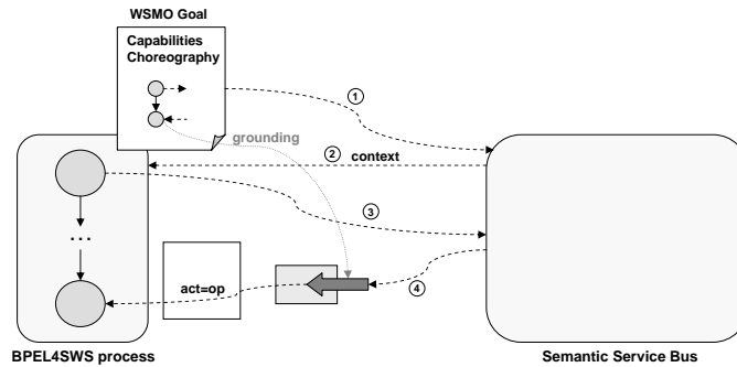
Figure 4. Asynchronous Invocation of a WSMO Web Service.
